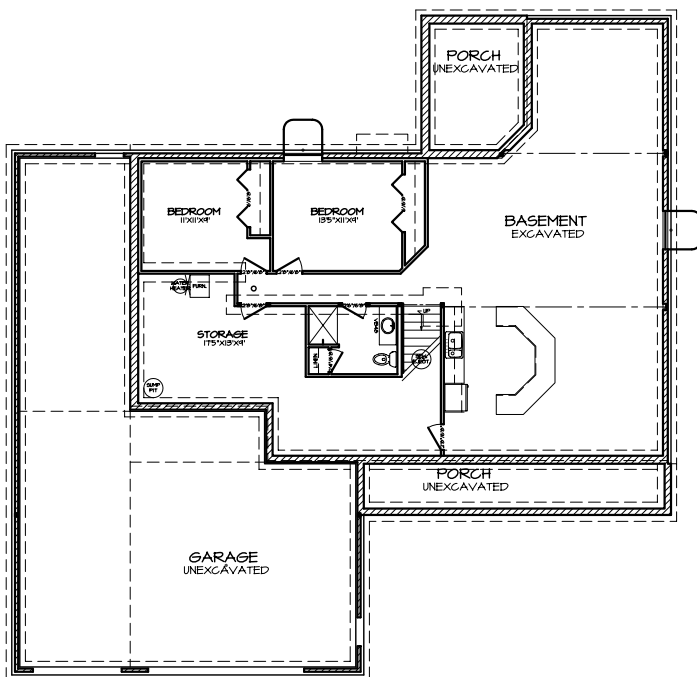
FOUNDATION PLAN A-3
