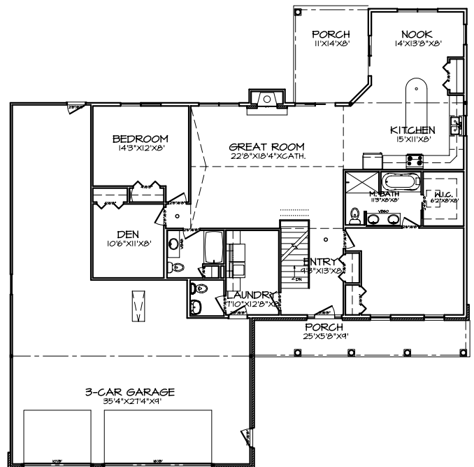
FIRST FLOOR PLAN A-4
